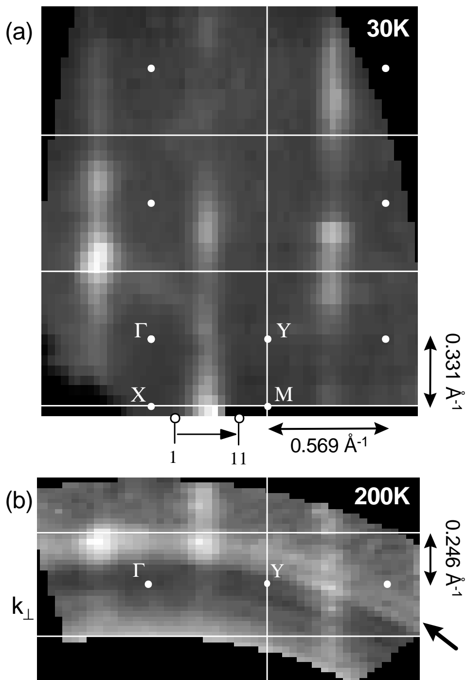
Figure 7.7: Near- E_F intensity map of \text{Li}_{0.9}\text{Mo}_6\text{O}_{17} . (a) k_{\parallel} plane projection for h\nu=24 eV with variation of two detector angles. (b) k_{\perp} / \Gamma -Y plane projection for varying h\nu=15 -32 eV and one detector angle. The thick arrow in (b) indicates the arc corresponding to h\nu=24 eV used in (a). In both maps, image contrast has been enhanced by dividing the data by the data heavily smoothed to retain only slowly varying cross-sectional dependences.
