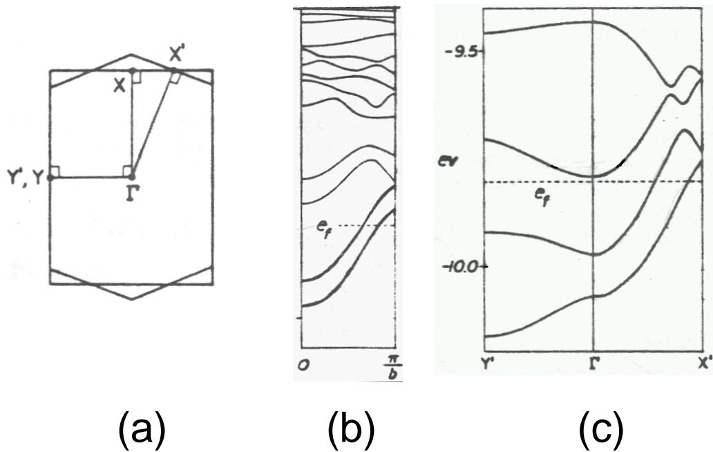
Figure 6.2: Band calculation for \text{K}_{0.3}\text{MoO}_3 , taken from Ref. [123]. (a) Brillouin zone for the \text{Mo}_{10}\text{O}_{30} slab. (b) Low lying d block bands for \text{Mo}_{10}\text{O}_{32} chain. (c) Low lying d block bands for \text{Mo}_{10}\text{O}_{30} slab.
