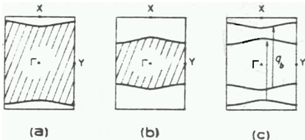
Figure 6.3: FS of \text{K}_{0.3}\text{MoO}_3 , calculated for the \text{Mo}_{10}\text{O}_{32} slab. From Ref. [123]. Shaded regions are occupied with electrons. (c) shows nesting of the two FS's.
