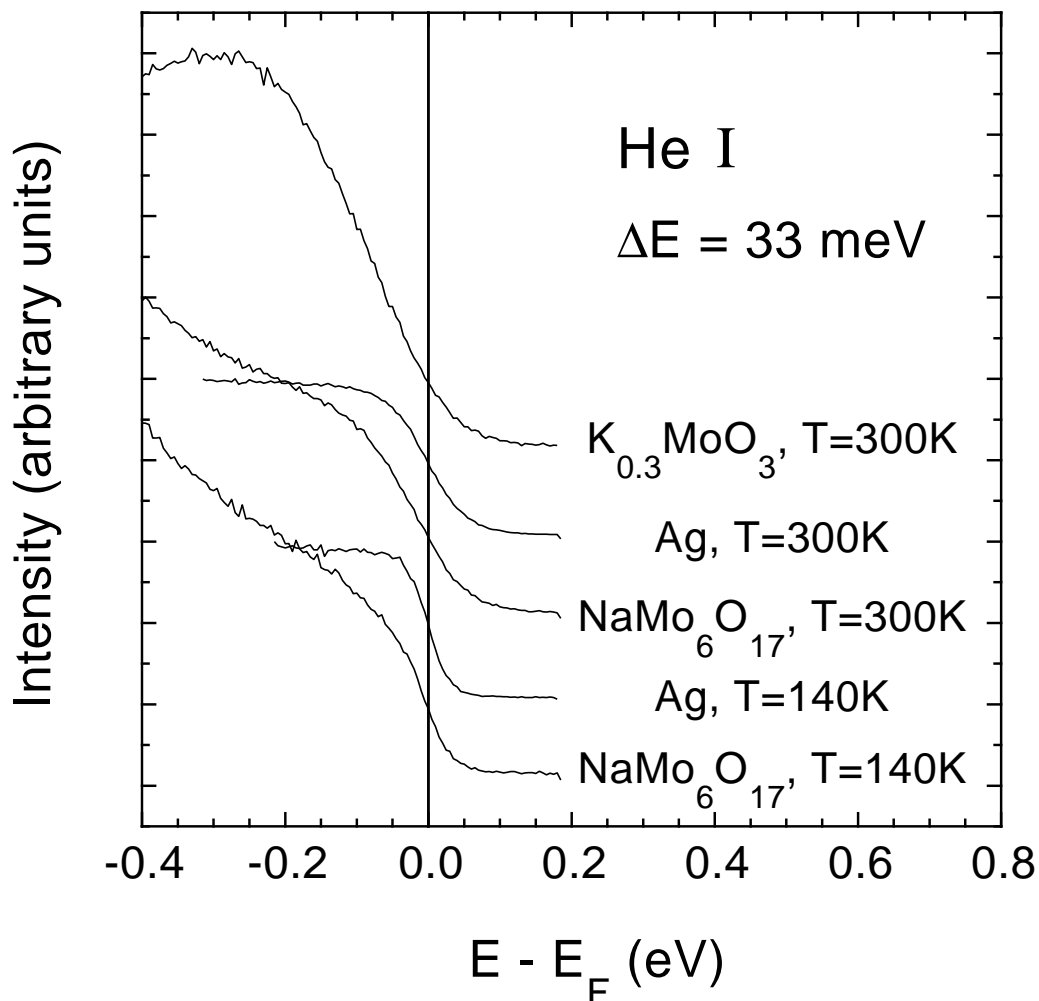
Figure 6.6: Angle integrated PES spectra of \text{K}_{0.3}\text{MoO}_3 and \text{NaMo}_6\text{O}_{17} taken at 300K and 140K. He I line (21.2eV) was used for the photon source. Overall instrumental energy resolution was 33meV FWHM. Spectra for Ag are shown for comparisons. Note the absence of a Fermi edge only for \text{K}_{0.3}\text{MoO}_3 .
