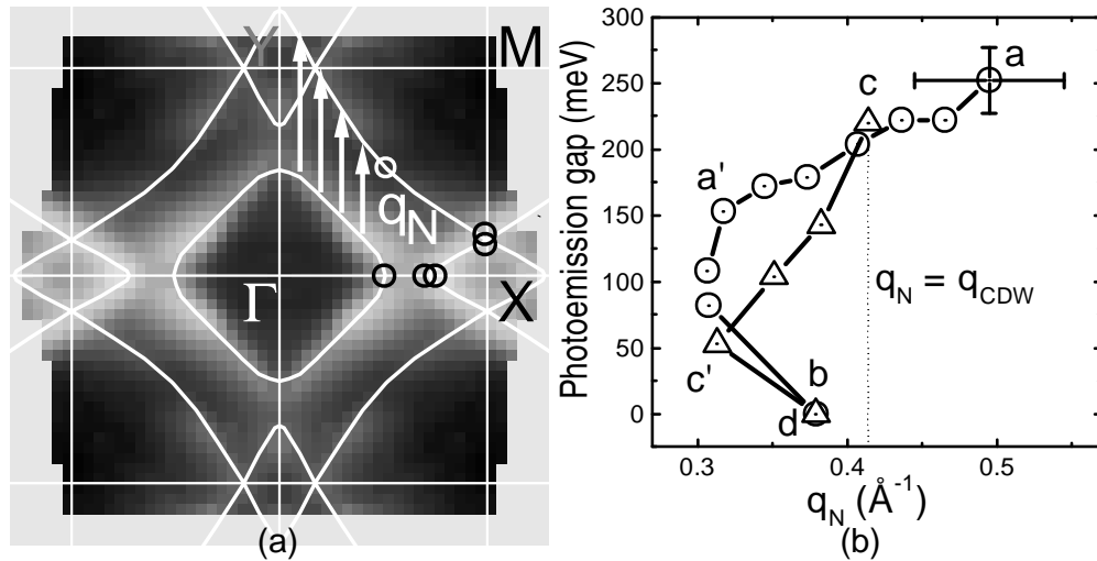
Figure 4.17: Experimentally deduced FS and gap anisotropy of \text{SmTe}_3 . (a) E_F crossing points (circles) from EDC's, experimental "FS" (white line), and nesting vectors ( q_N ), connecting "FS" pieces plotted over the E_F intensity map. (b) Electron removal gaps on the two "FS" pieces plotted as a function of q_N . The gap values are taken from the data of Fig. 4.16 (c). Representative error bars are shown.
