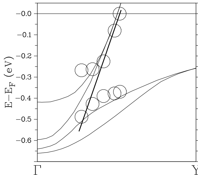
Figure 7.9: ARPES dispersions near E_F crossing for \text{Li}_{0.9}\text{Mo}_6\text{O}_{17} . Band theoretical calculation (Fig. 7.2, scaled by 2.5) is shown for comparison. The circles correspond to peak positions extracted from spectra 2 to 6. Thick line, to be used later for lineshape modeling, shows a linear approximation of the dispersing feature.
